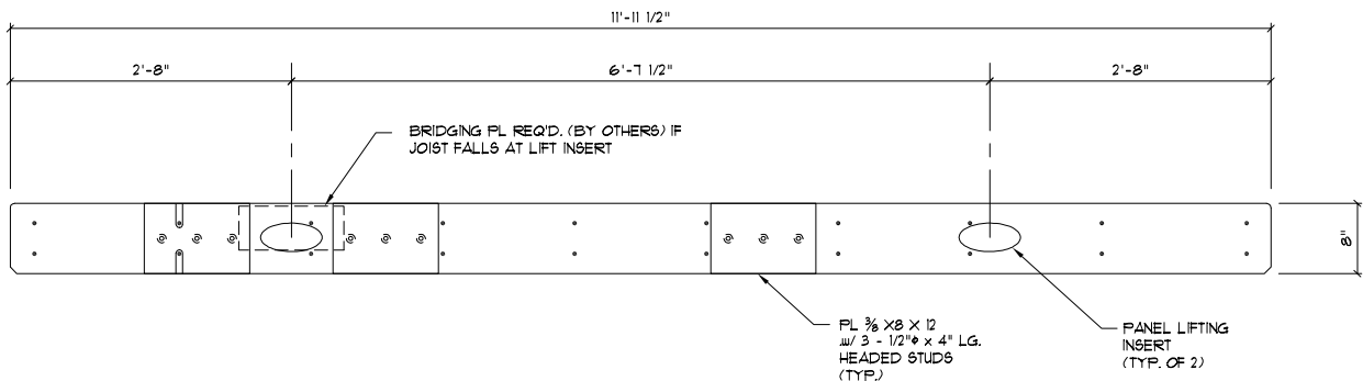
12' PANEL TOP VIEW FOR JOIST BEARING
