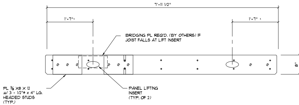
8' PANEL TOP VIEW FOR JOIST BEARING
