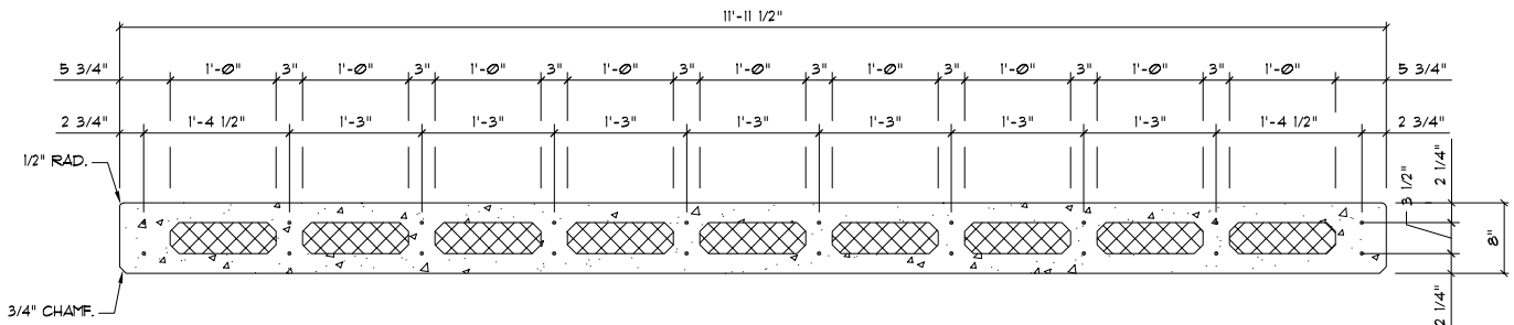
12' STANDARD PANEL CROSS SECTION
