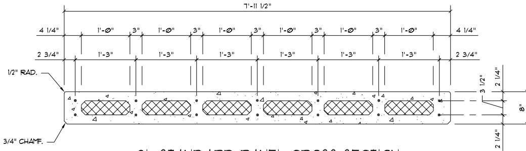
8' STANDARD PANEL CROSS SECTION
