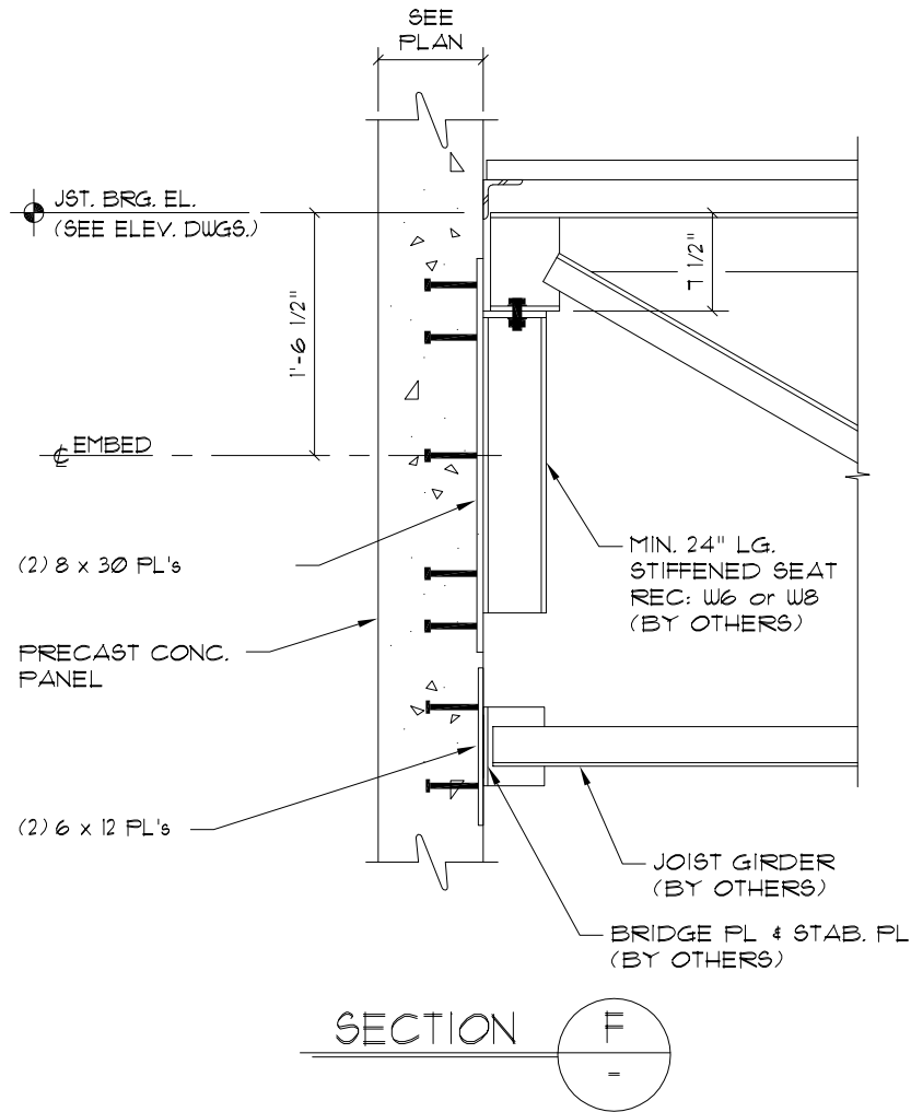
JOIST GIRDER SUPPORT AT PANEL JOINT
