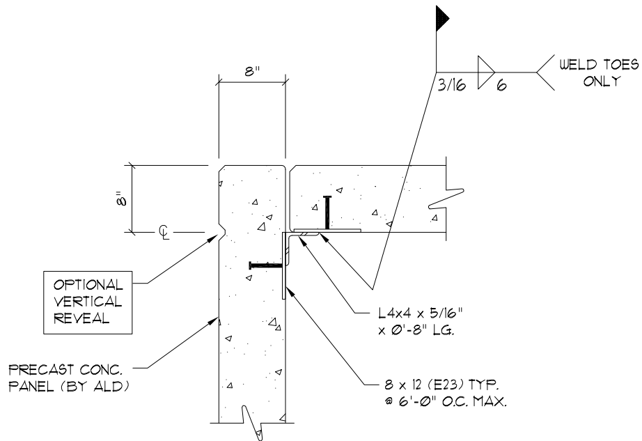
TYPICAL CORNER CONNECTION
