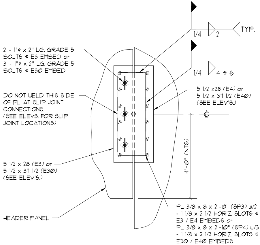
TYPICAL HEADER-TO-PANEL CONNECTION
