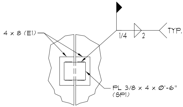
TYPICAL PANEL-TO-PANEL CONNECTION
