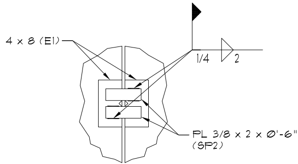
TYPICAL PANEL-TO-PANEL SLIP JOINT CONNECTION
